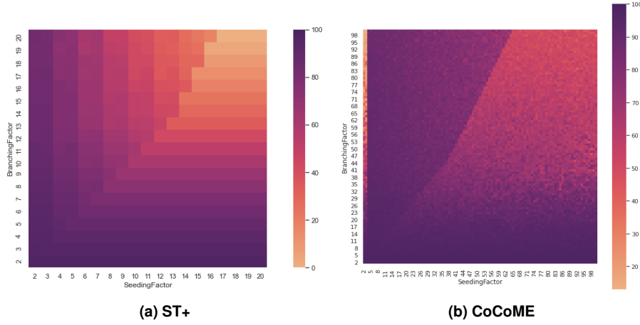
Figure 7. Tree pruning ( P ) for different branching ( B ) and seeding ( S ) factors.
