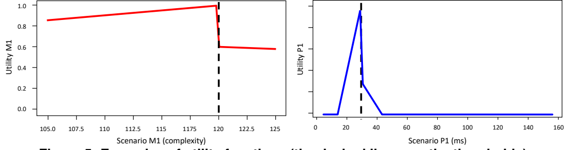
Figure 5. Examples of utility functions (the dashed lines are the thresholds).
