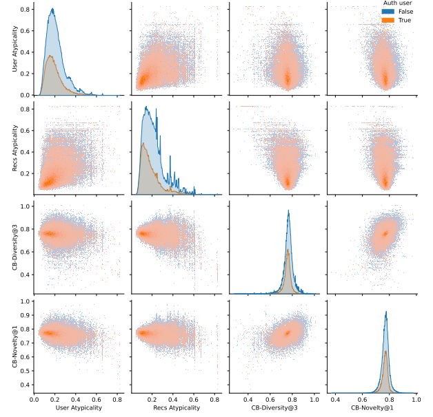
Figure 2: Atypicality, cb-diversity, and cb-novelty.
